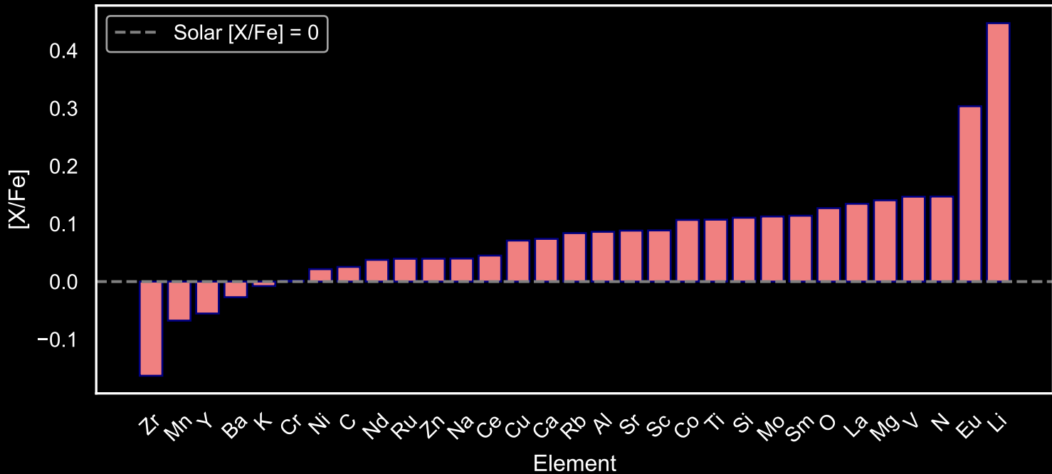
Abundance Pattern for GALAH Star Field [7] (N=292)
