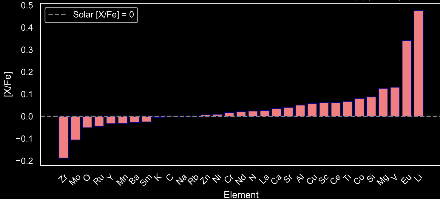
Abundance Pattern for GALAH Main Sequence Stars: Star Field [7] (N=130)
