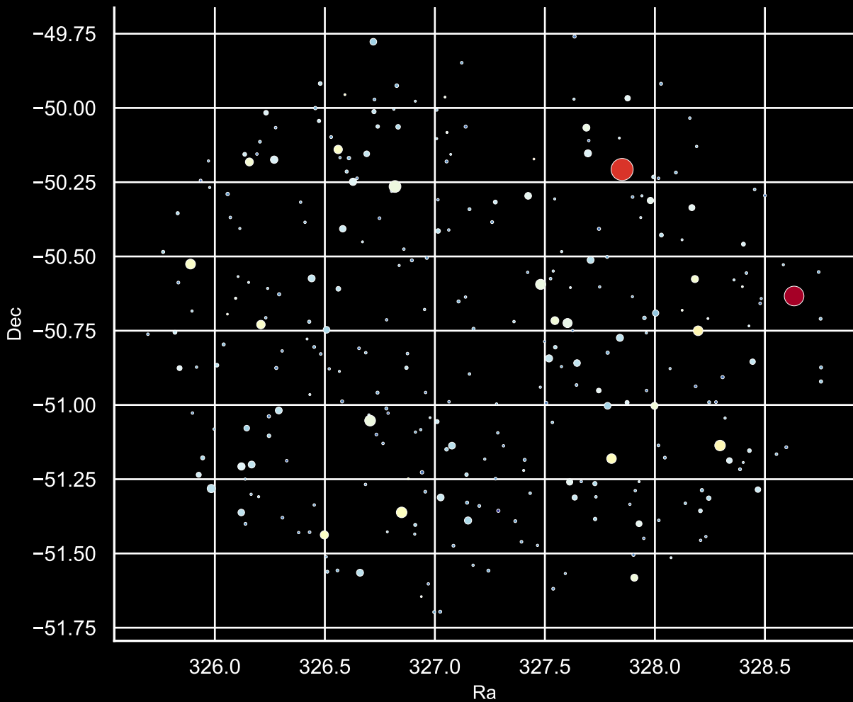
Field [7] Ra [327.18] Dec [-50.78] Stars: 292
