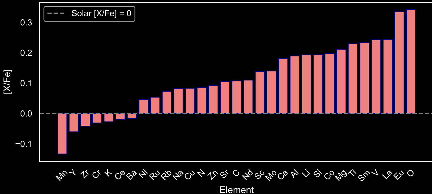
Abundance Pattern for GALAH Red Giants: Star Field [7] (N=73)
