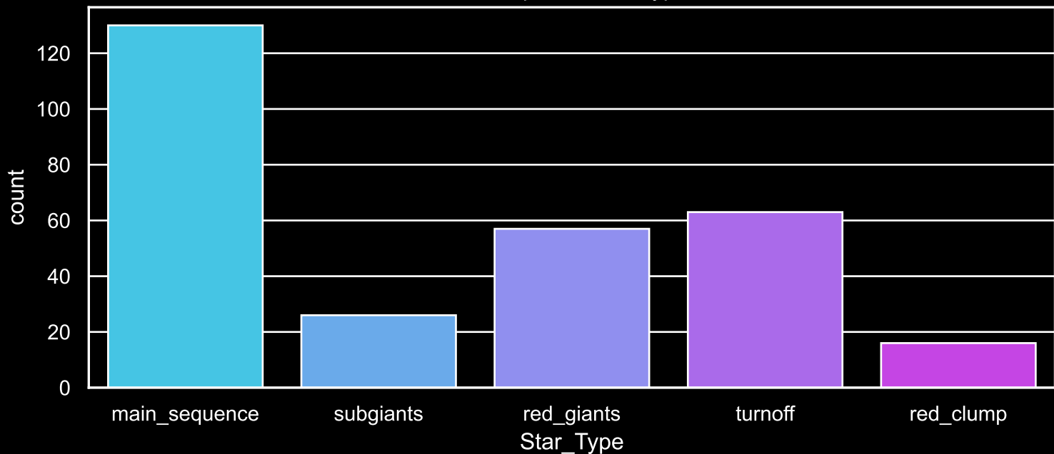
Field [7] Count plot of Star Type
